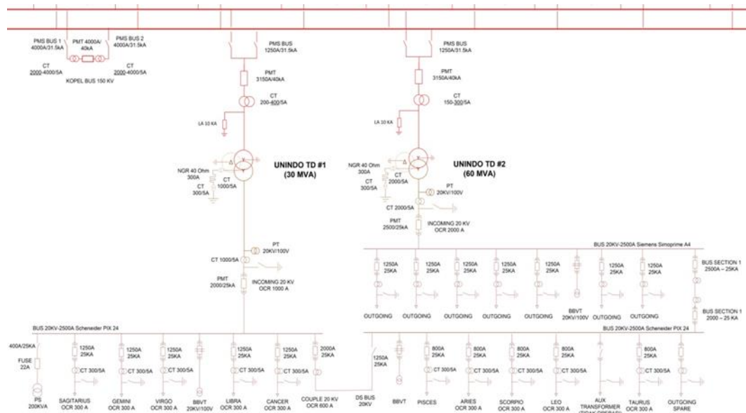
Gambar 2. Single Line Gardu Induk Lahat
